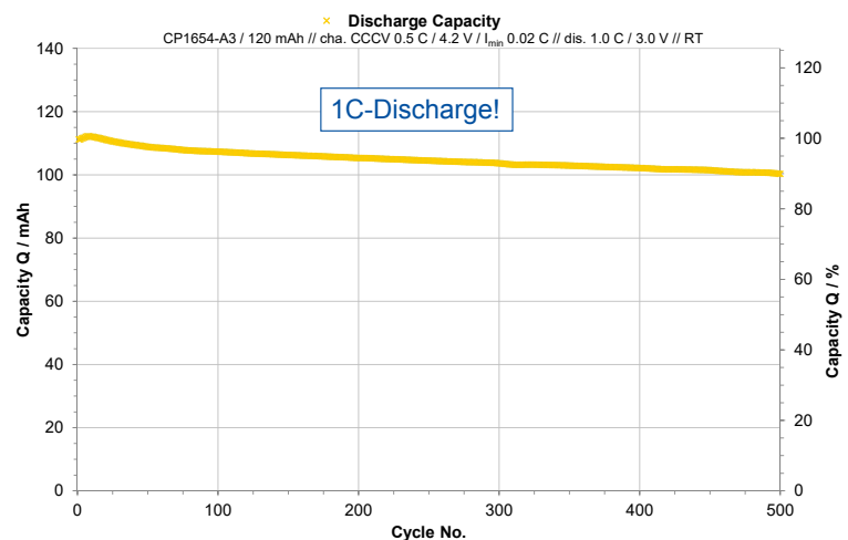
CoinPower CP1654 A3 Discharge Performance – 0.5C/1C
