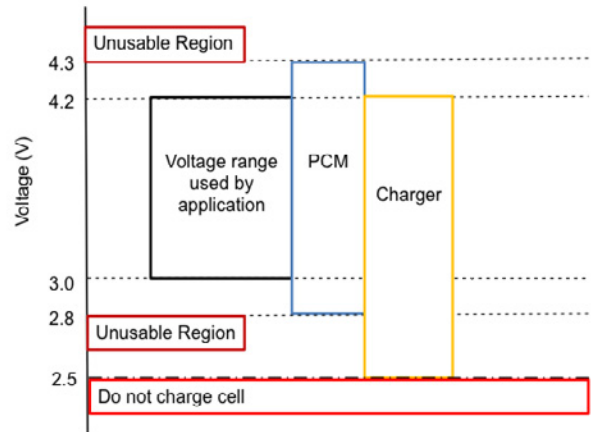
Voltage range for PCM and Charger
