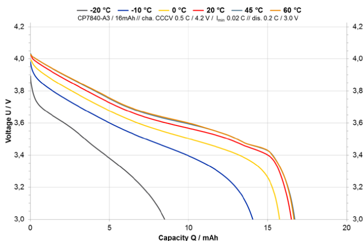
CP7840 A3 – Discharge Characteristic at various temperature
