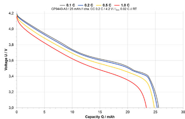
CP9440 A3 – Discharge Characteristic with different loads
