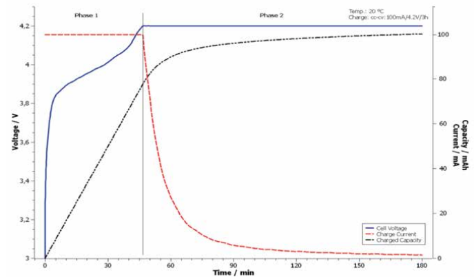
Illustrates the different phases during a charge cycle
