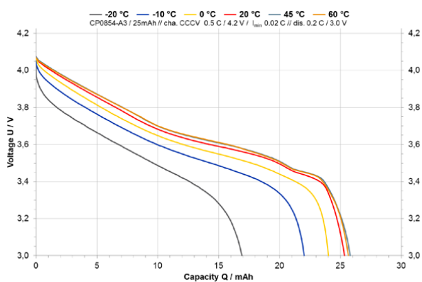
CP0854 A3 – Discharge Characteristic at various temperatures
