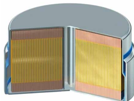
Construction of VARTA CoinPower
