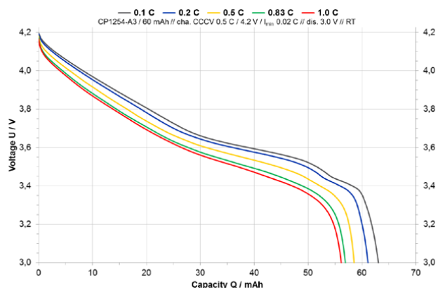
CP1254 A3 – Discharge Characteristic with different loads
