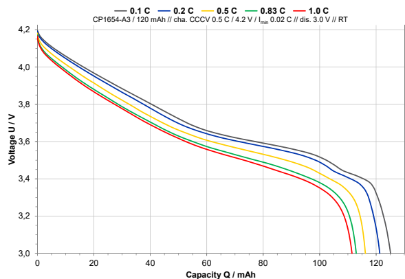
CP1654 A3 – Discharge Characteristic with different loads
