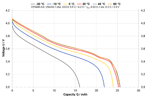
CP9440 A3 – Discharge Characteristic at various temperatures
