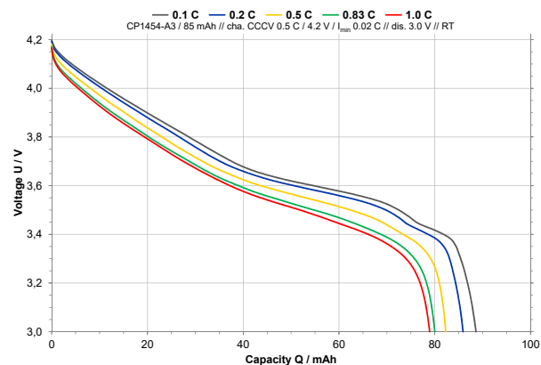
CP1454 A3 – Discharge Characteristic with different loads
