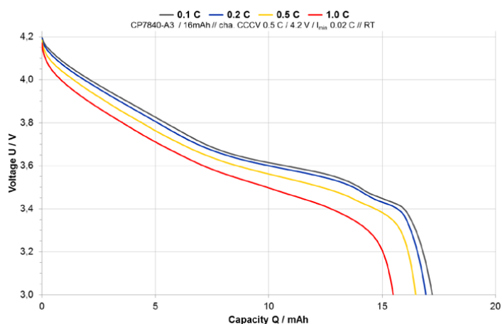
CP7840 A3 – Discharge Characteristic with different loads
