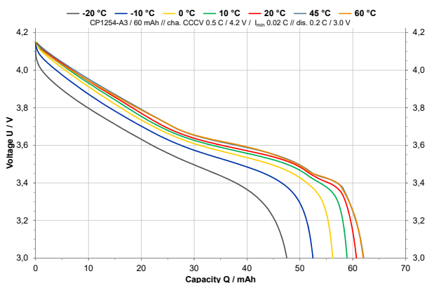
CP1254 A3 – Discharge Characteristic at various temperature
