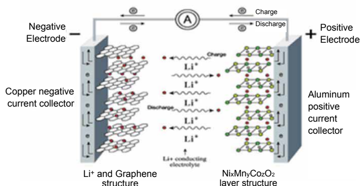
Chemical reaction in Li-Ion rechargeable battery
