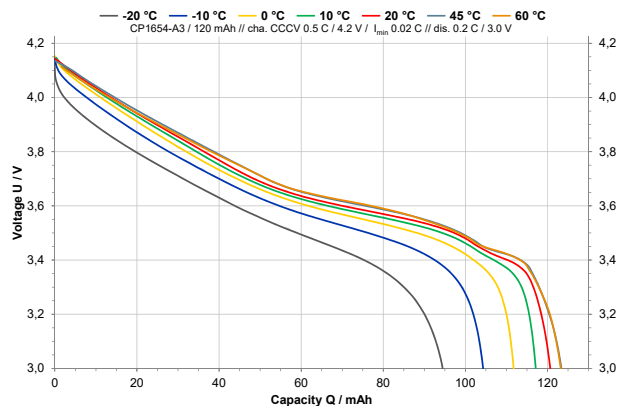
CP1654 A3 – Discharge Characteristic at various temperatures
