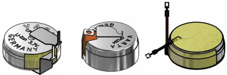
Examples for different battery assemblies
