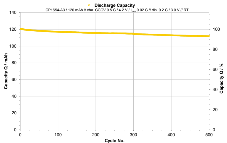
CoinPower CP1654 A3 Discharge Performance – 0.5C/0.2C
