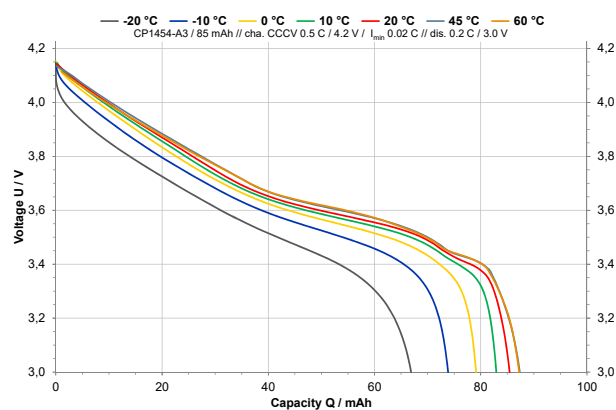
CP1454 A3 – Discharge Characteristic at various temperatures
