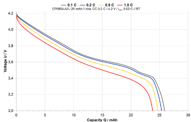
CP0854 A3 – Discharge Characteristic with different loads
