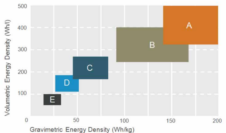
FIG. 1 Comparison of different rechargeable battery systems
